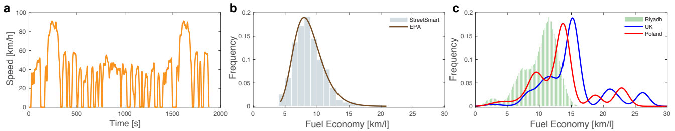
Figure 2: (a) FTP-75 EPA’s standard speed profile used for calculating the reported inner-city fuel economies of cars. (b) The distribution of fuel economies recreated by the StreetSmart model shows the same distribution as that of the reported fuel economies. (c) The distribution of fuel economies based on Riyadh’s fleet of cars compared to those of Poland and the UK shows that the distributions are similar but shifted from one another. The car fleet of Riyadh is less fuel efficient than that of Poland which is less than that of the UK
