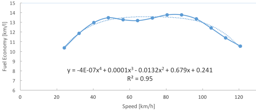
Figure 1: A fitted model of fuel economy vs. speed from DOE as a baseline comparison to the StreetSmart model. [28]
