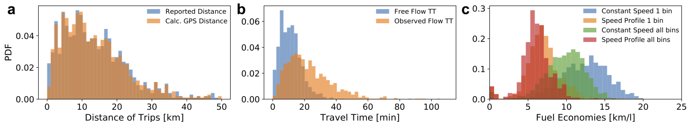
Figure 4: Data Verification figures using trips in the morning peak time period of weekdays from 8 - 9 AM. (a) Histogram of Reported and calculated Trip Distances. (b) Histogram of free flow travel time and Observed travel time in matched trips. (c) Histogram of Fuel economies using constant speed, speed profiles, and 1 bin and all bins.
