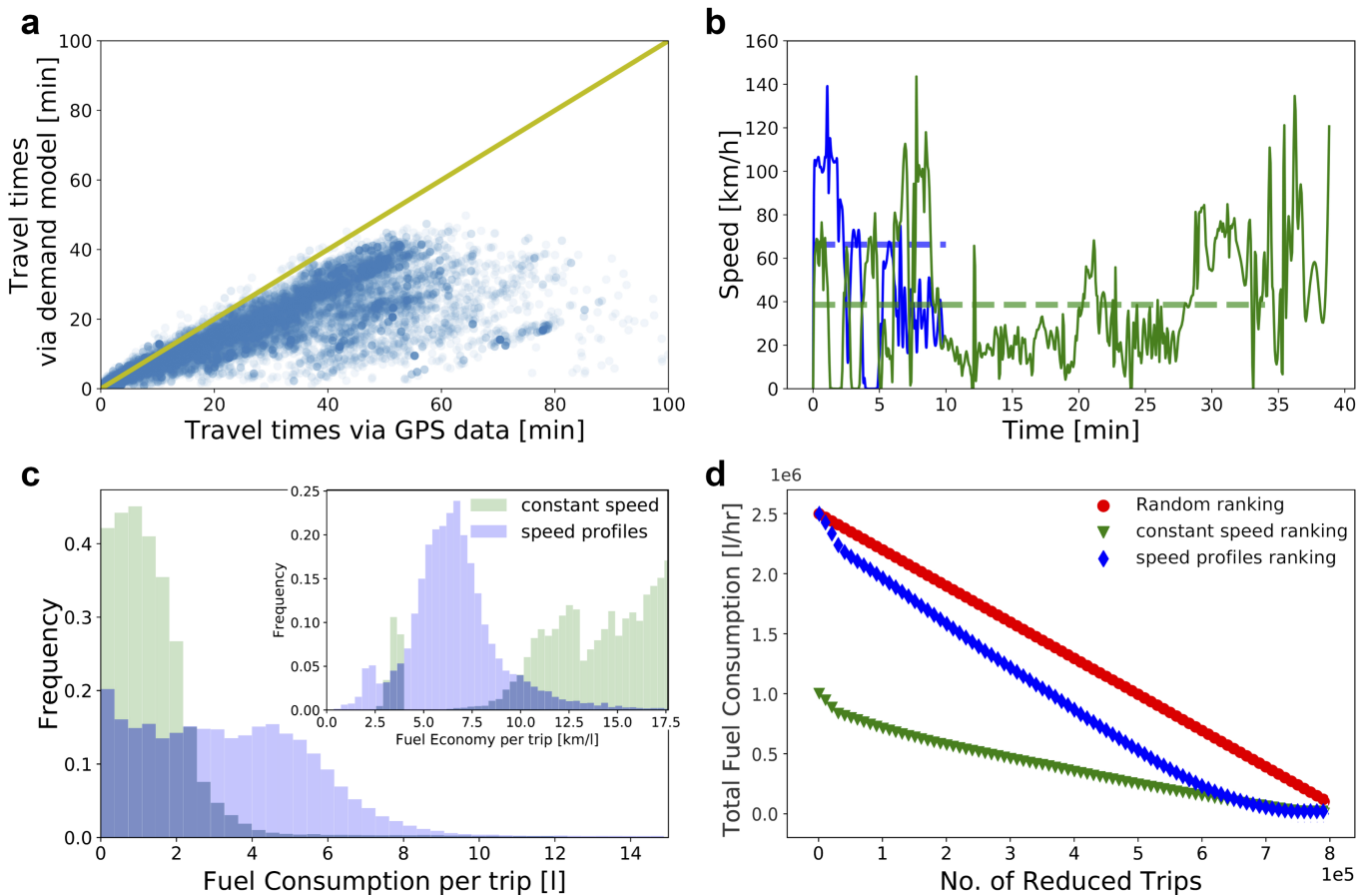
Figure 6: Fuel consumption estimates at urban scale. (a) Comparison of the travel time of the routes in the constant speed model via travel demand vs. the input used in our method using GPS data (b) Sample speed profiles in two routes used to estimate fuel consumption overlaid with the constant speed used for comparison (c) Estimates of fuel consumption and fuel economy in the morning peak via our method (speed profiles) and the base line method (constant speed) (d) Random and targeted fuel savings vs. number of reduced trips.
